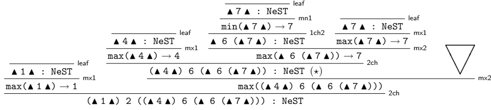
Figure 8: Abbreviated proof tree
