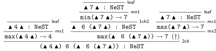
Figure 9: Abbreviated proof tree after the first question
